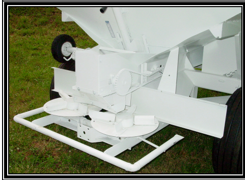
Gearbox Driven Dual Spinners
