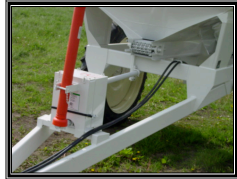
PTO Driven Spinners – 540 or 1000 RPM
