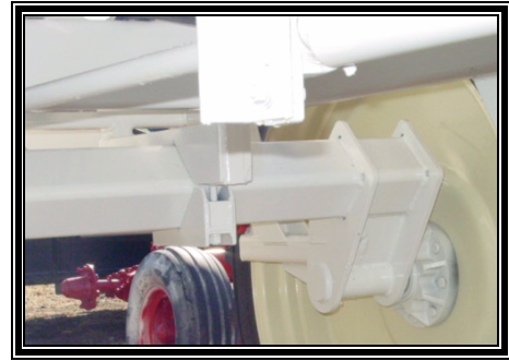
Heavy-duty 8-bolt hubs and 3-3/8" Spindle
