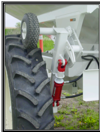
Stainless Steel Box Legs and 8" Apron Chain
