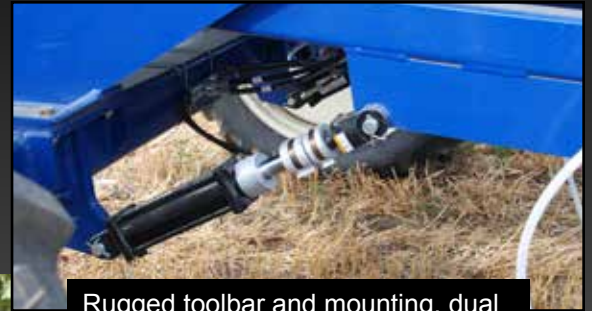
Rugged toolbar and mounting, dual 3 x 8 lift cylinders with depth setting spacers; 3 x 20 wing fold cylinders
