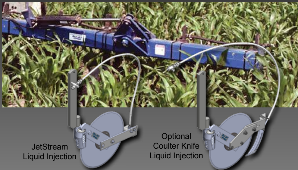
Rugged toolbar and mounting, dual 3 x 8 lift cylinders with depth setting spacers; 3 x 20 wing fold cylinders
